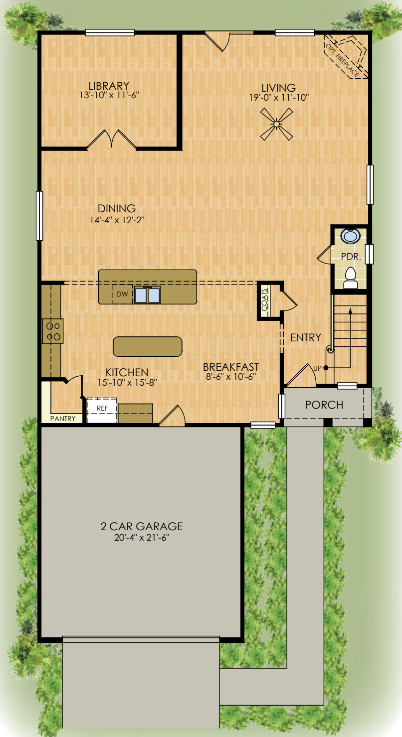
FIRST FLOOR
